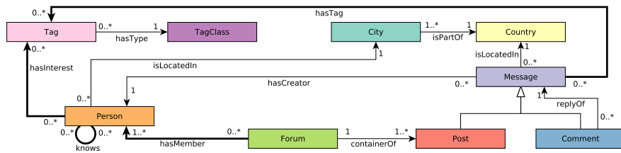
(a) Graph schema visualized using a UML-style notation. Edge labels with many-to-many cardinality are depicted with thick lines. The knows edge labels represent undirected edges, while the rest of the edges are directed.
