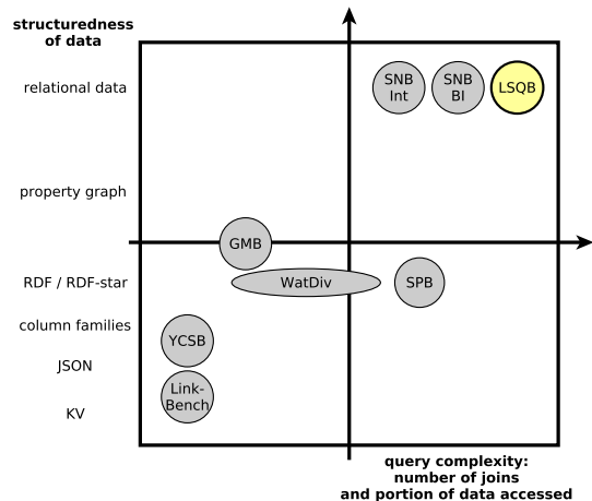
Figure 1: Landscape of DB benchmarks according to query complexity and data structuredness. The benchmark proposed in this paper, LSQB, is highlighted.
