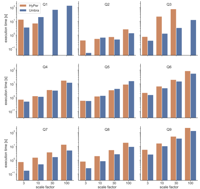
Figure 4: Query execution times on scale factors 3, 10, 30, and 100 for HyPer and Umbra, the two best performing systems under benchmark.
